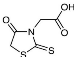
Fig. 1: Rhodanine-3-acetic acid
